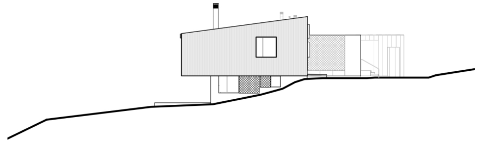
EAST ELEVATION
