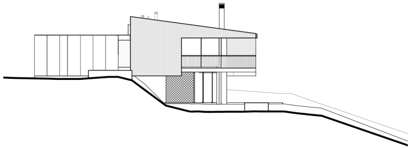
WEST ELEVATION
