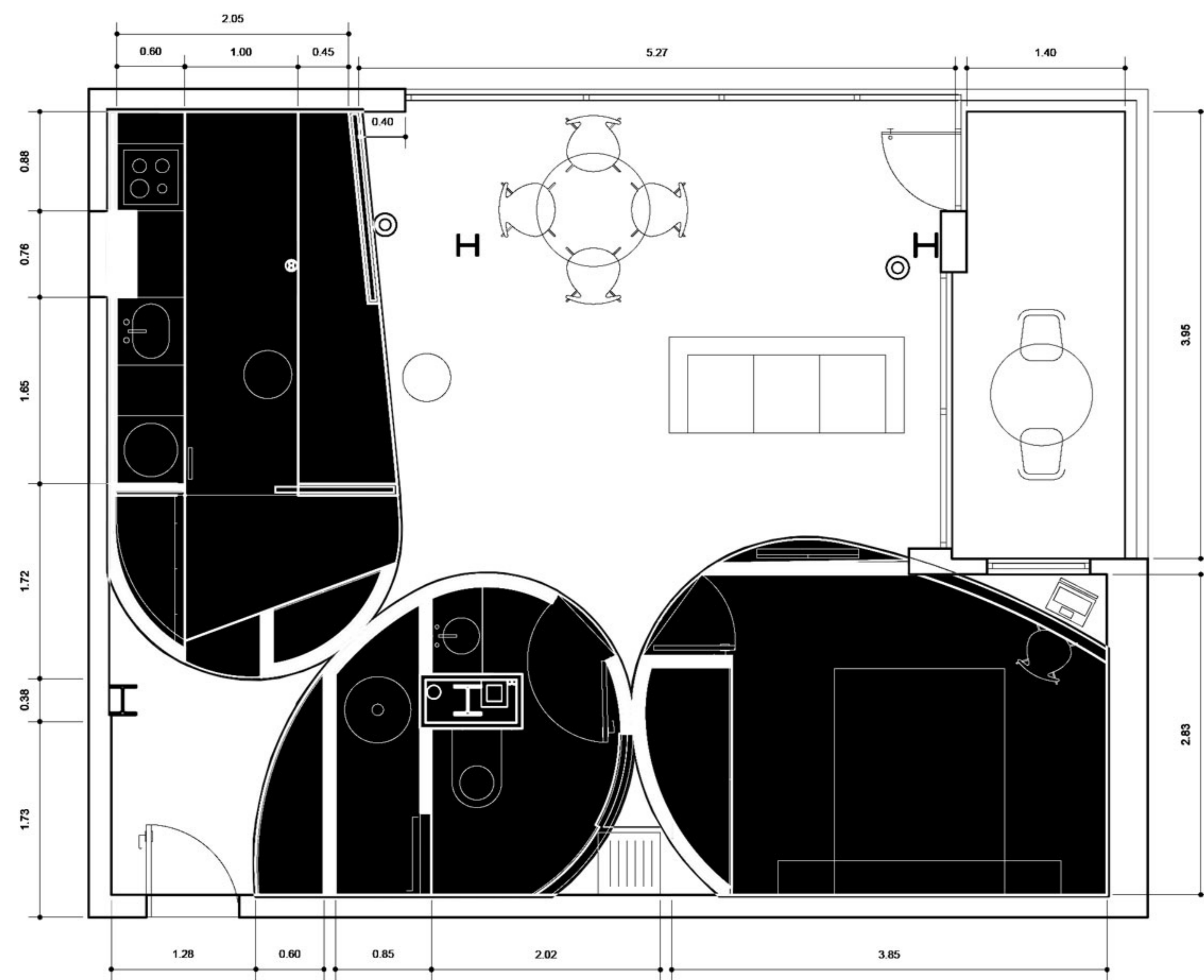
Foam House, Pedro Pitarch, 2026
