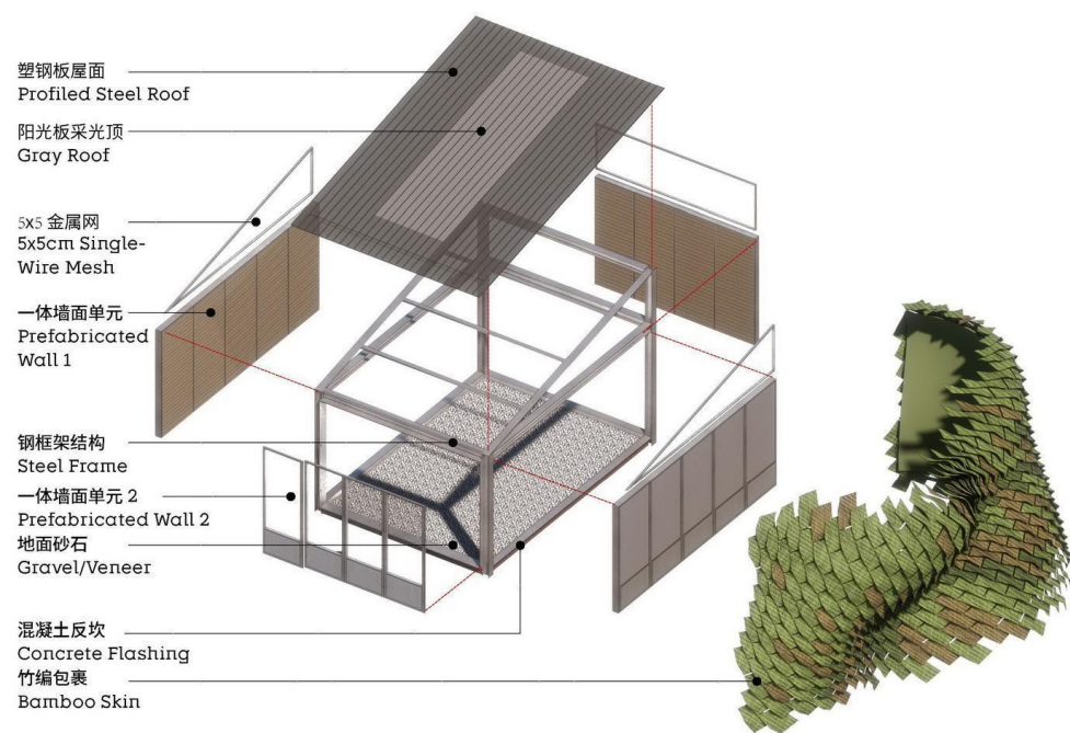
1 鸟舍单元模块化建造 Aviary Units Modular Construction
