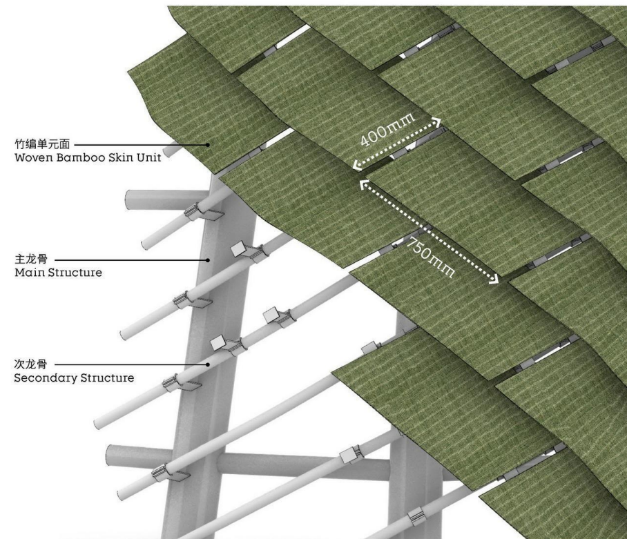
2 竹编构造示意 Bamboo weaving Construction Diagram
