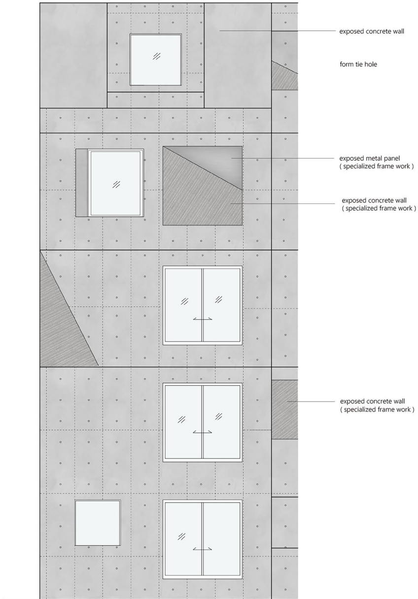
PARTIAL DETAIL ELEVATION
