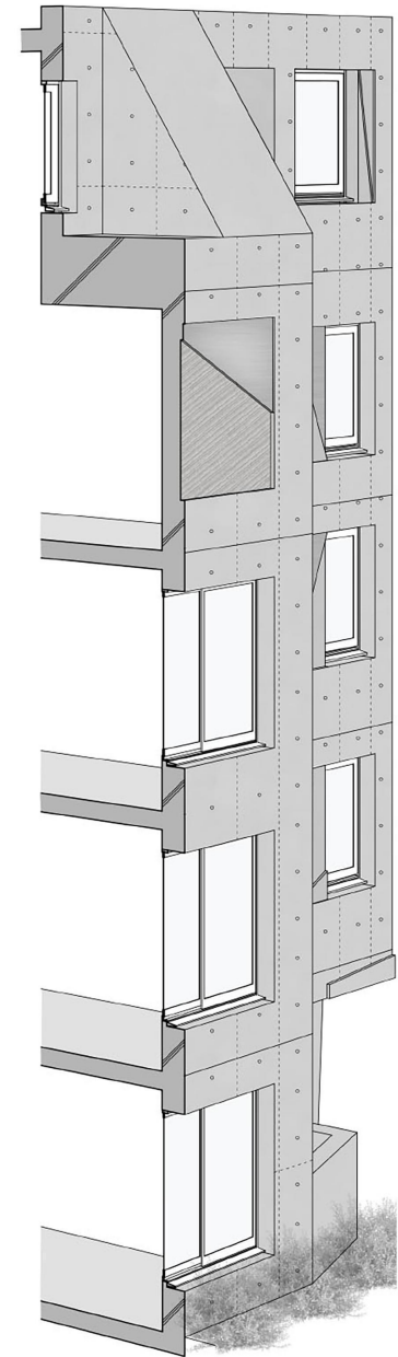
PARTIAL SHIFTING WALL PERSPECTIVE
