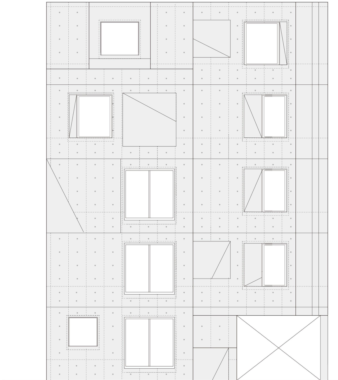
SOUTH ELEVATION
