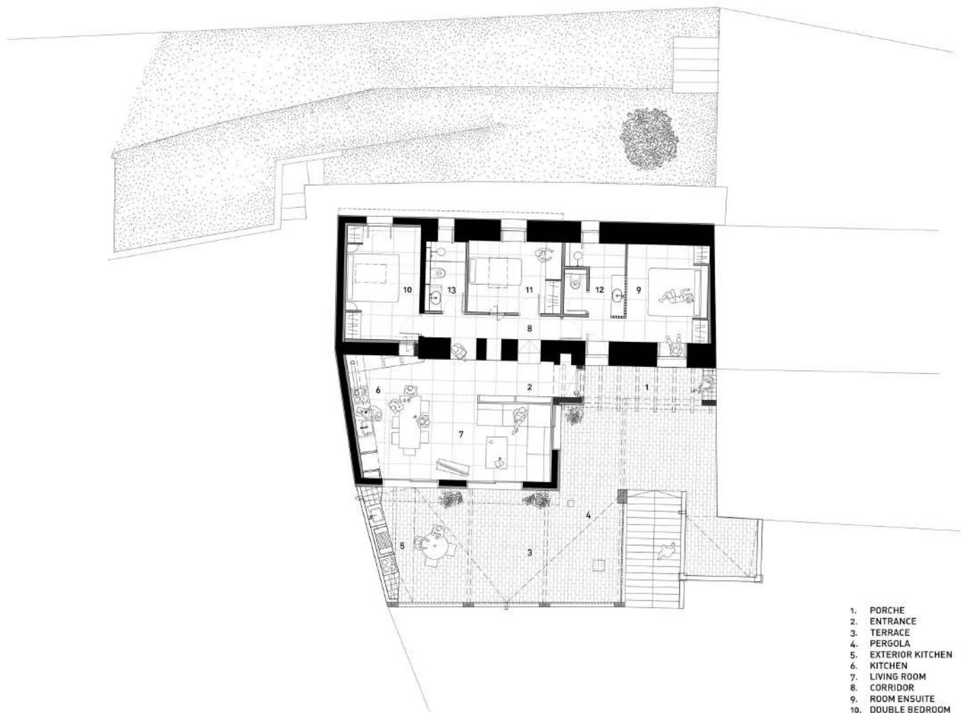
FLOORPLAN
